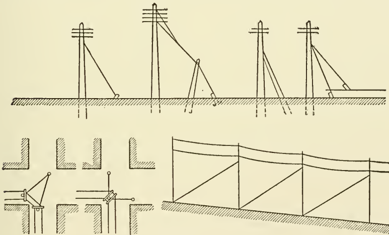
Fig. 33. Methods of Guying Poles
